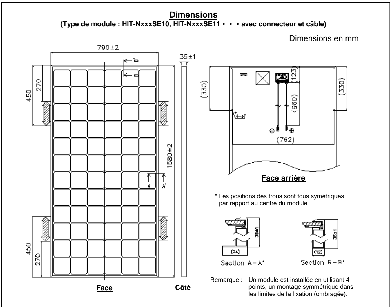
Figure 2-1: Dimensions
