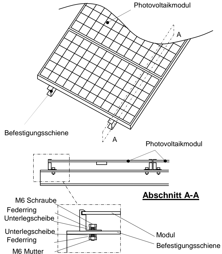
Abb. 1: Installation
